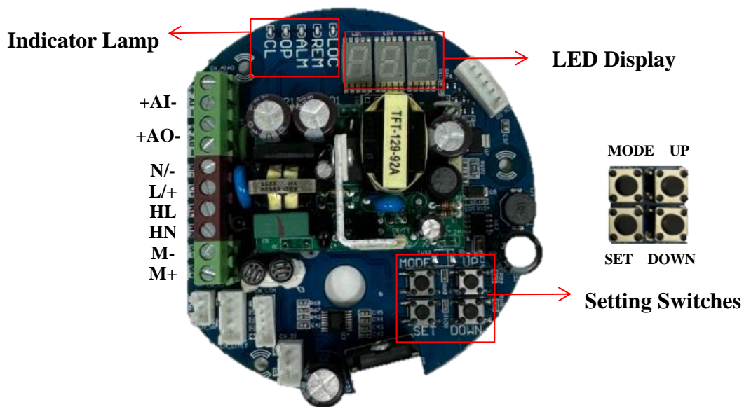
Modulating Control Board
